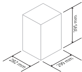
PACKAGING DIMENSIONS
